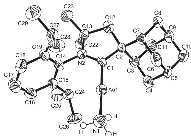
Figure 1. Molecular structure of complex B in the solid state. (Hydrogen atoms, except those at N1, and the (C_6F_5)_4B anion are omitted for clarity; ellipsoids are drawn at 50% probability).
